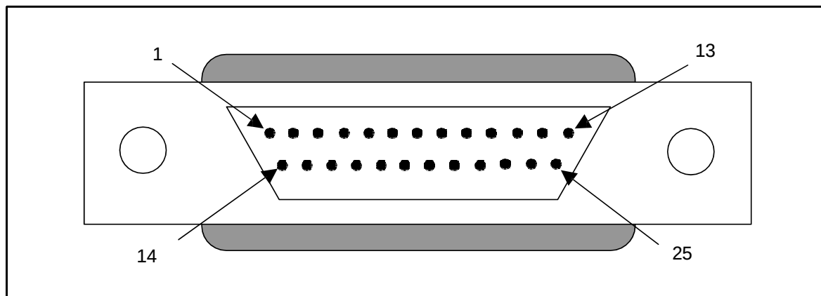
Figure 15-16. DB-25 Connector
