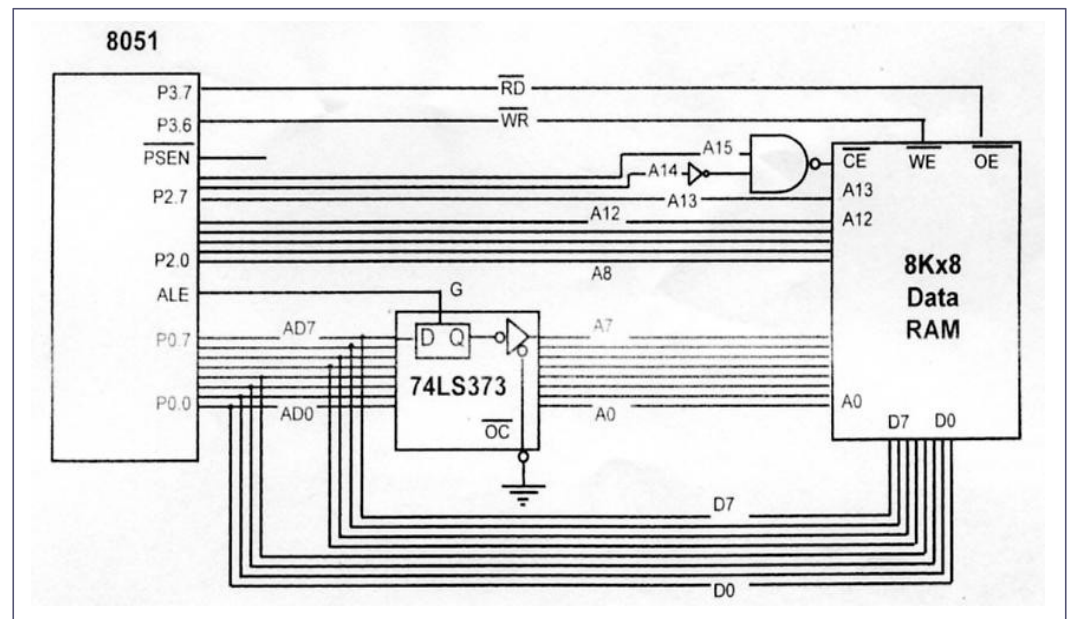
8051 Connection to External Data RAM
