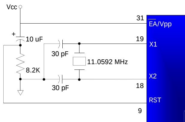
Power-on RESET circuit
