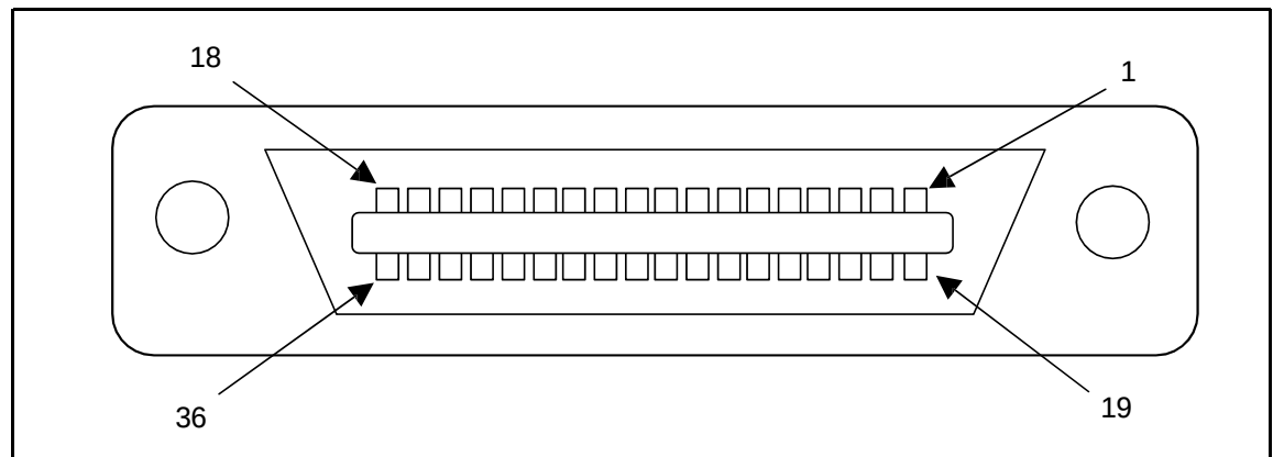
Figure 15-17. 36-Pin Centronics Connector
