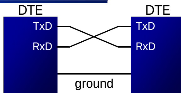
Null modem connection
