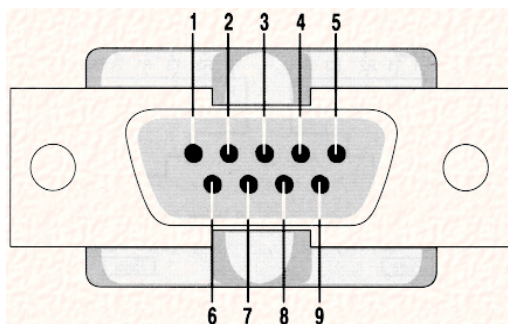
RS232 Connector DB-9
