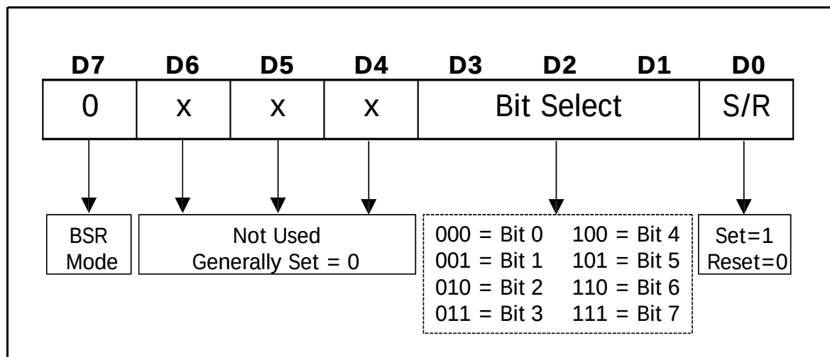
Figure 15-12. BSR Control Word
