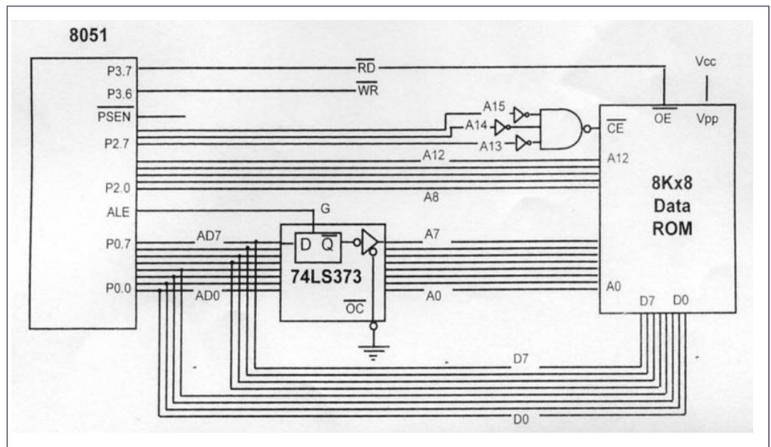
8051 Connection to External Data ROM
