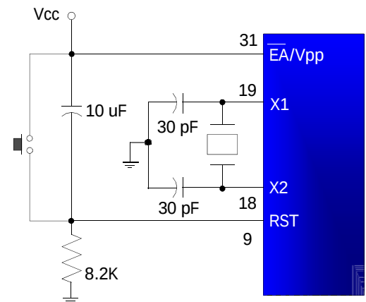
Power-on RESET with debounce
