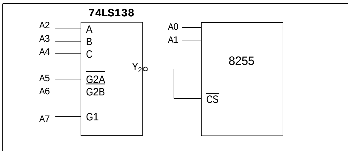
Figure 15-7. 8255 Decoding Using 74LS138
