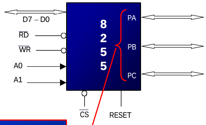
8255 Block Diagram
